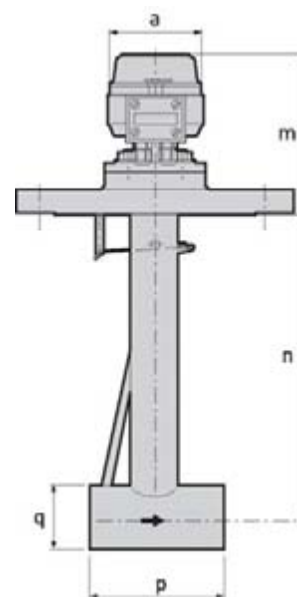
DW 184 non-Ex/Exi side view
