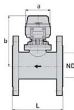
DW 183 non-Ex / Exi side view
