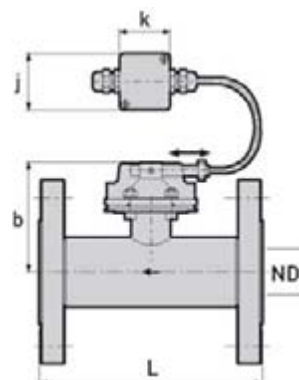
DW 182 HT side view
