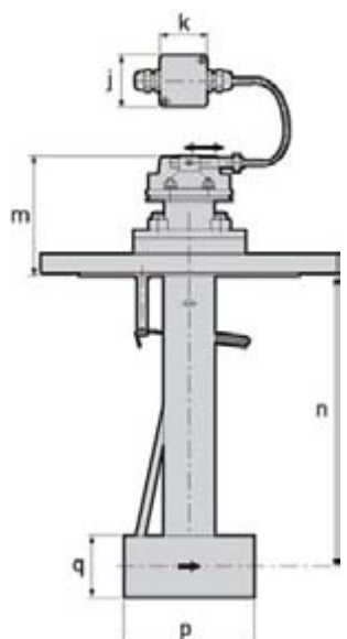
DW 184 HT side view
